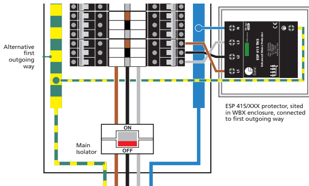
Figure 2: ESP 415/XXX Protector connected to the nearest available outgoing (MCB) way to the incoming supply. Since there is insufficient space within the distribution board the ESP Protector has been mounted within a separate enclosure, directly alongside the board.
